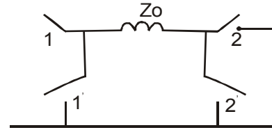
Switching diagram
